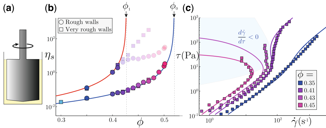
Fig. 5 Rheological data fitting procedure. a Cylindrical-Couette geometry used to characterize the rheology of the aqueous suspension of cornstarch (yellow). The gray area represents the cylinder rotating in the direction indicated by the black arrow. b Viscosity (Pa.s) below ( \tau \ll \tau^* ) and above ( \tau \gg \tau^* ) the shear-thickening transition versus \phi . Blue-solid-line: frictionless branch, red-solid-line: frictional branch, black-dashed-lines: jamming volume fractions for the frictionless and frictional branches defining \phi_0 and \phi_1 , respectively. Square and circle symbols correspond to measurements performed with different wall roughness. The data points made transparent are not used in the fitting procedure as for these points, the measurement depend on the wall roughness. c Shear stress \tau versus shear rate \dot{\gamma} measured at various volume fraction \phi . Solid lines: Wyart & Cates rheological laws. The blue shaded area highlights the region where the rheograms are negatively sloped ( d\dot{\gamma}/d\tau < 0 ).
